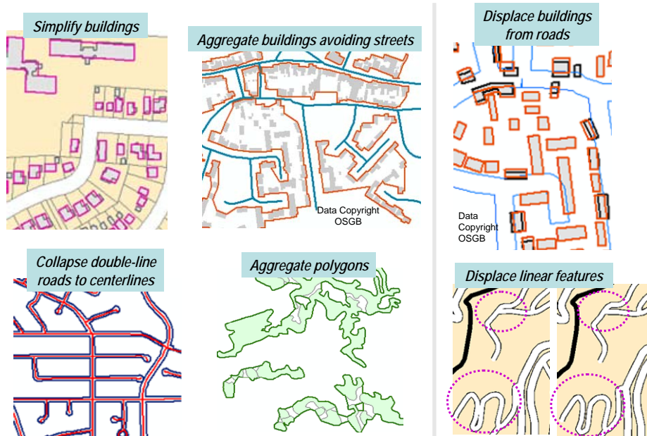
Fig 13. Generalization Algorithms
