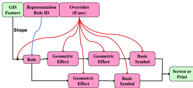
Fig. 2 - Drawing pipeline for representations
