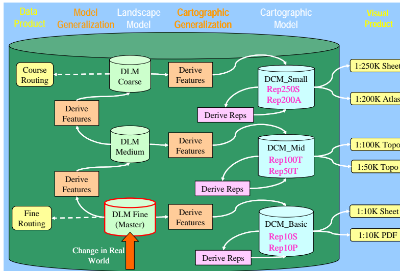
Fig. 11 - Multi-scale DLM/DCM Data Flows.
